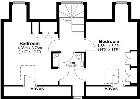
Second Floor Approx. 51.9 sq. metres (559.1 sq. feet)
