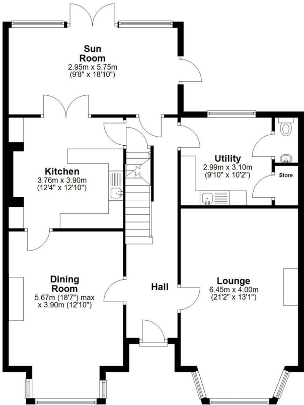
Ground Floor Approx. 104.1 sq. metres (1120.7 sq. feet)
